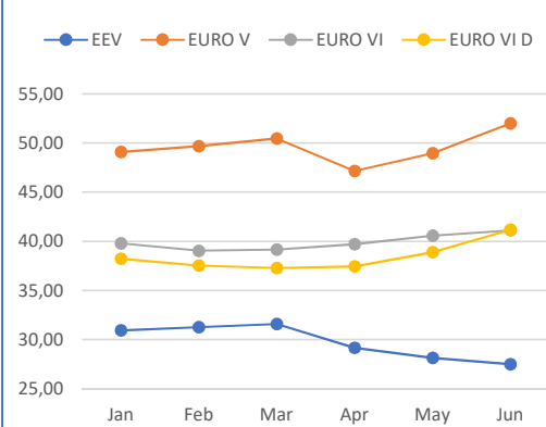
Consumption l/100 km by vehicle type
