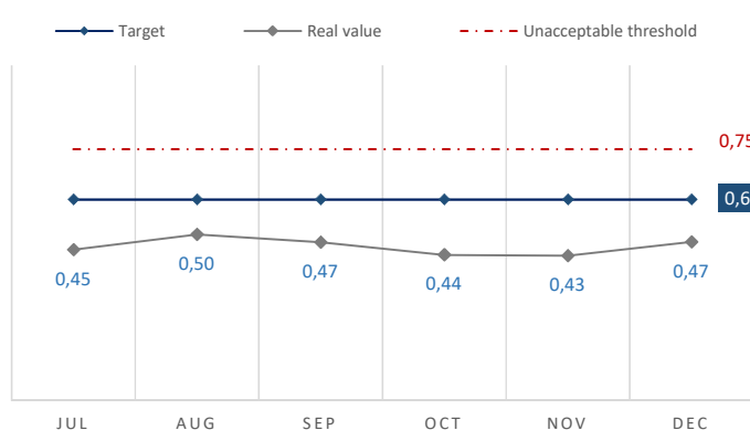
Fuel consumption in units (l)/travelling persons per month
