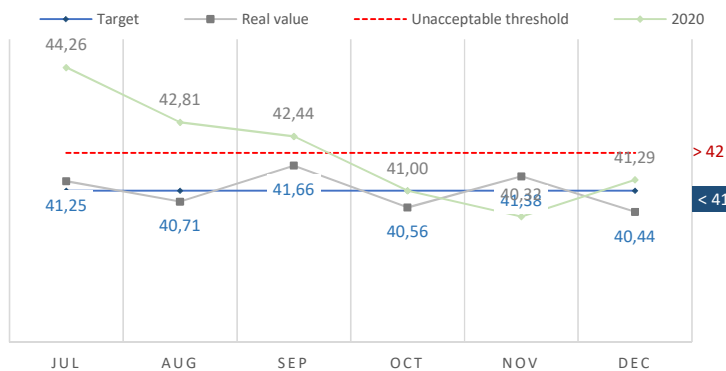
Fuel consumption in units (l)/100km
